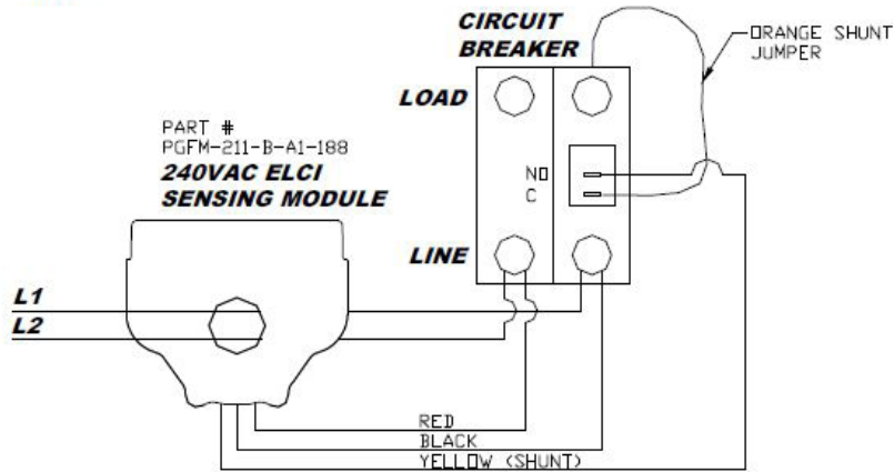
SINGLE PHASE 240VAC (L1, L2, GRND)
