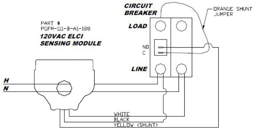
SINGLE PHASE 120VAC (HOT, NEUTRAL, GRND)
