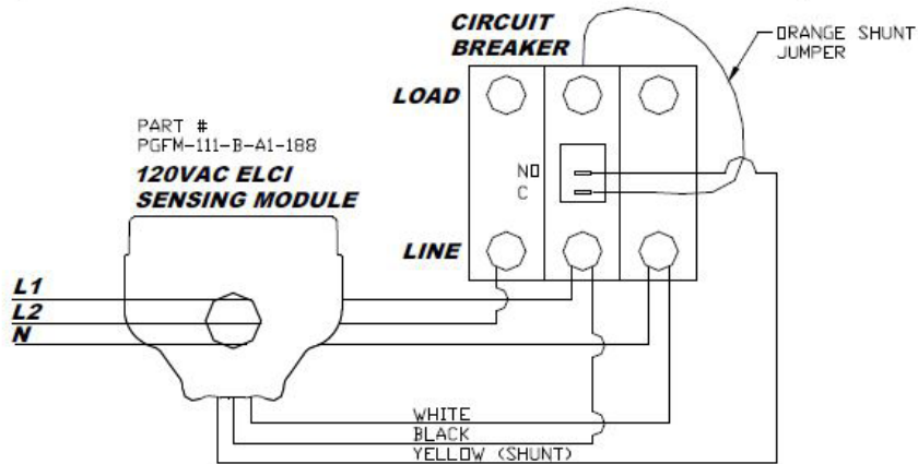
SPLIT PHASE 120/240VAC BREAKING NEUTRAL (L1, L2, N, GRND)
