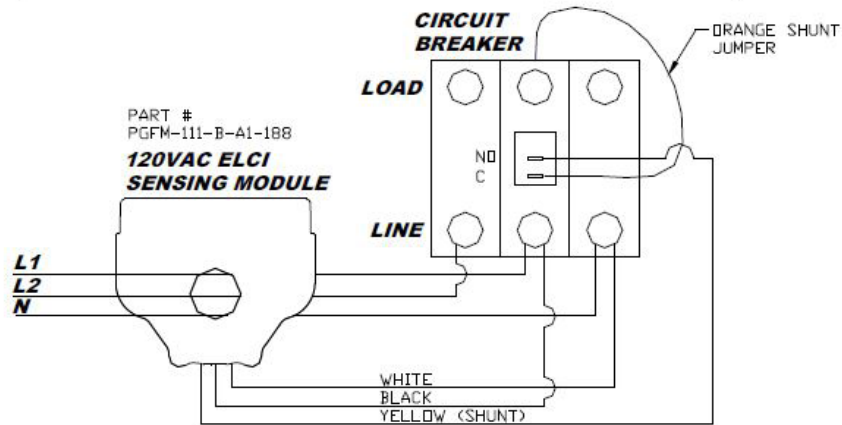
SPLIT PHASE 120/240VAC BREAKING NEUTRAL (L1, L2, N, GRND) GRND
