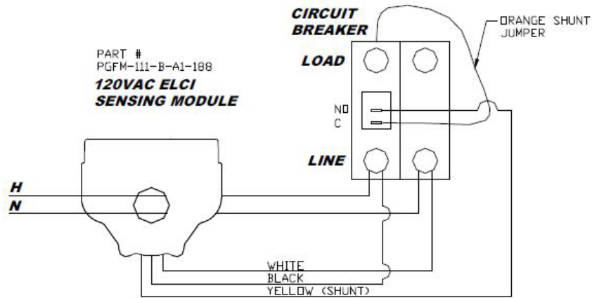
SINGLE PHASE 120VAC (HOT, NEUTRAL, GRND) GRND
