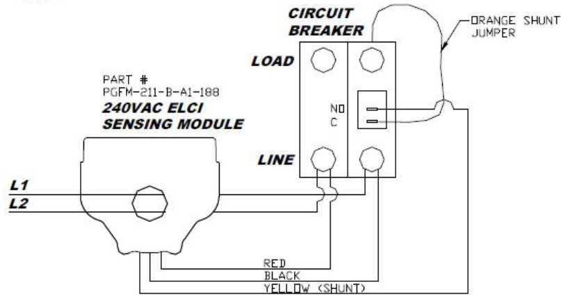
SINGLE PHASE 240VAC (L1, L2, GRND) GRND
